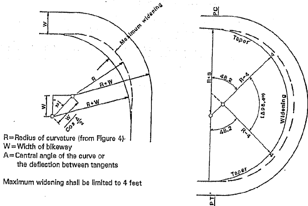
Figure 2: CURVE WIDENING Source: State of Oregon
