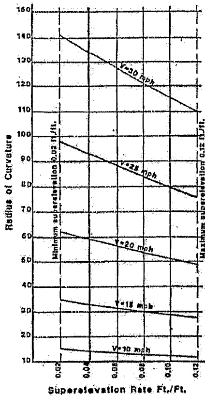
Figure 1: STANDARD SUPERELEVATION FOR BIKEWAYS Source: State of Oregon
